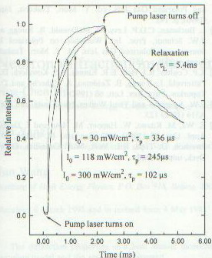
Fig. 5. The Faraday rotation signal for pump laser light intensities of 300, 118 and 30 mW/cm 2 . The traces show three distinct regions. The first displays the increase of the rotation signal as the pump beam turns on and \theta increases with the polarization of the K vapor. The time to polarize the vapor is seen to decrease with increasing pump light intensity. The second region shows a sharp transient feature of 50–60 \mu s duration. The third region shows a slow relaxation of \tau_L = 5.4 ms.
