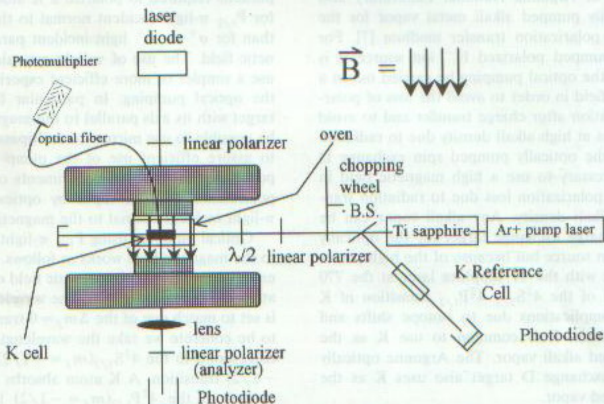
Fig. 2. Schematic diagram of experimental apparatus.
